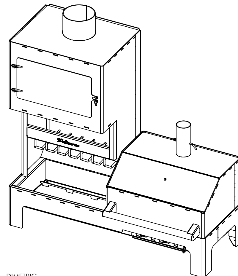
DIMETRIC
