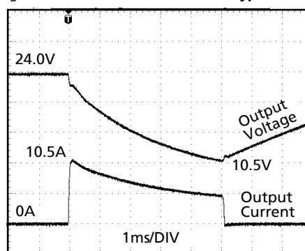
Fig. 27-2 Peak load 10.5A for 5ms, typ.
