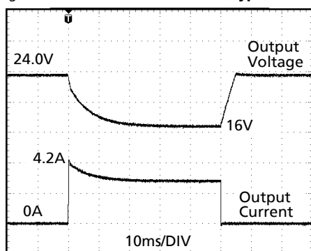
Fig. 27-1 Peak load 4.2A for 50ms, typ.
