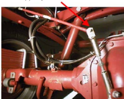
Upper joint of the LSV –rod
