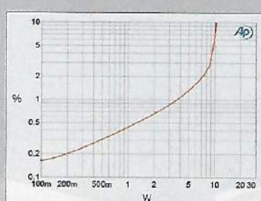
Fig.5 Air Tight ATM-300R, 8 ohm tap, both channels driven, distortion (%) vs 1kHz continuous output power into 8 ohms.
