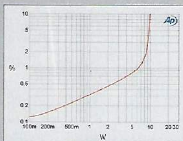
Fig.7 Air Tight ATM-300R, 4 ohm tap, both channels driven, distortion (%) vs 1kHz continuous output power into 4 ohms.
