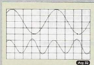
Fig.9 Air Tight ATM-300R, 8 ohm tap, 1kHz waveform at 1Wpc into 8 ohms, 0.44% THD+N (top); distortion and noise waveform with fundamental notched out (bottom, not to scale).
