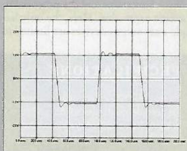
Fig.2 Air Tight ATM-300R, 4 ohm tap, small-signal, 10kHz squarewave into 8 ohms.
