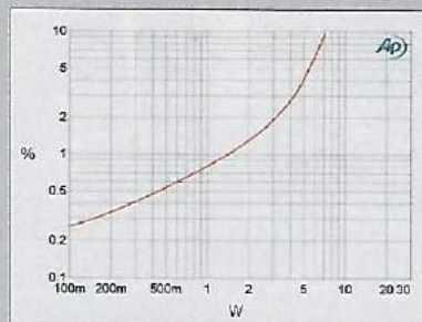
Fig.6 Air Tight ATM-300R, 8 ohm tap, both channels driven, distortion (%) vs 1kHz continuous output power into 4 ohms.
