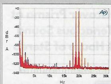
Fig.11 Air Tight ATM-300R, 8 ohm tap, HF intermodulation spectrum, DC-30kHz, 19+20kHz at 1Wpc peak into 8 ohms (linear frequency scale).
