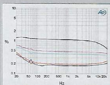
Fig.8 Air Tight ATM-300R, 8 ohm tap, THD+N (%) vs frequency at 1V into: 8 ohms (left channel blue, right red), 4 ohms (left cyan, right magenta), 2 ohms (left gray).
