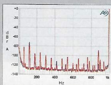
Fig.4 Air Tight ATM-300R, 8 ohm tap, spectrum of 1kHz sinewave, DC-1kHz, at 1W into 8 ohms (linear frequency scale).
