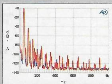
Fig.10 Air Tight ATM-300R, 8 ohm tap, spectrum of 50Hz sine wave, DC-1kHz, at 1Wpc into 8 ohms (linear frequency scale).
