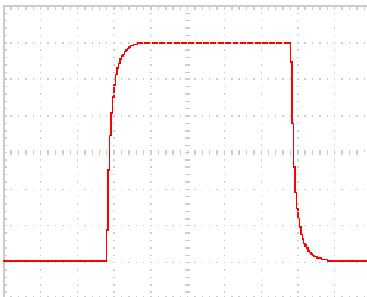
28 WATT SQUARE WAVE AT 10 KHZ
