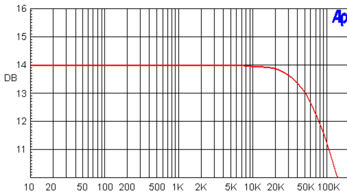
RESPONSE VS FREQUENCY
