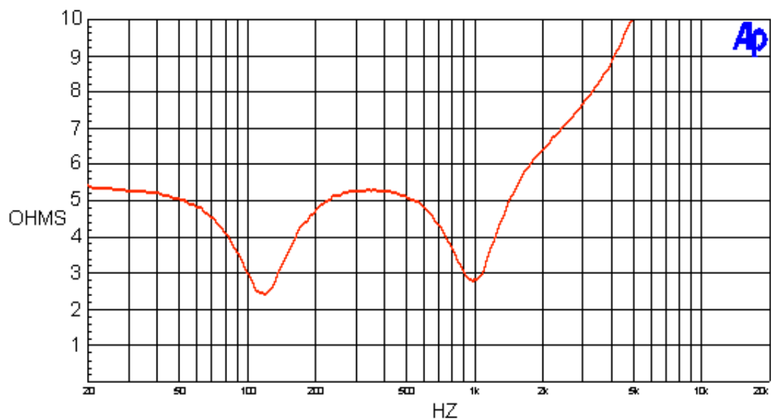
IMPEDANCE OF TOUGH LOAD
