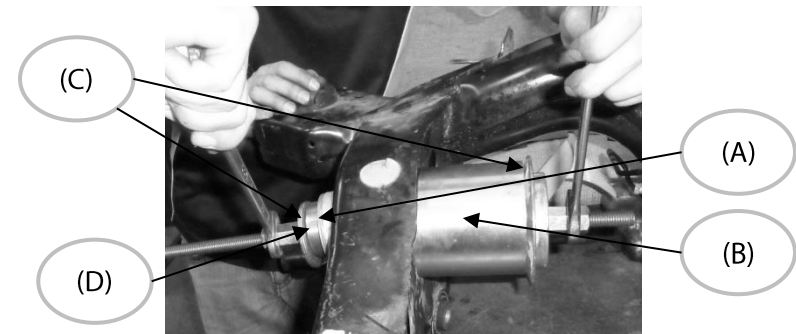
Tools setup for factory bushes removal
