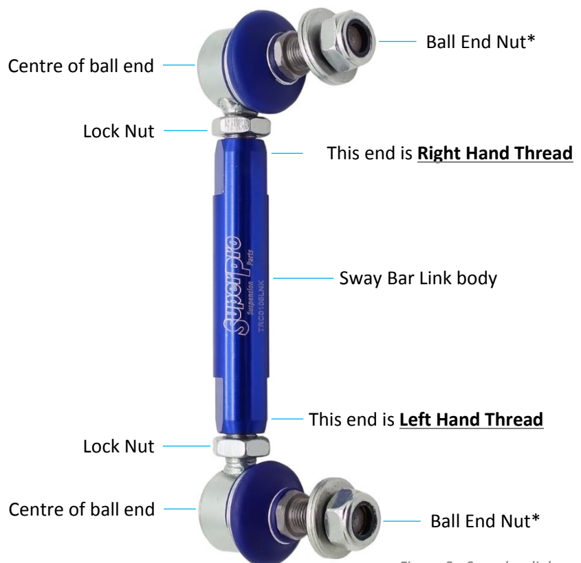
Figure 2 - Sway bar link
