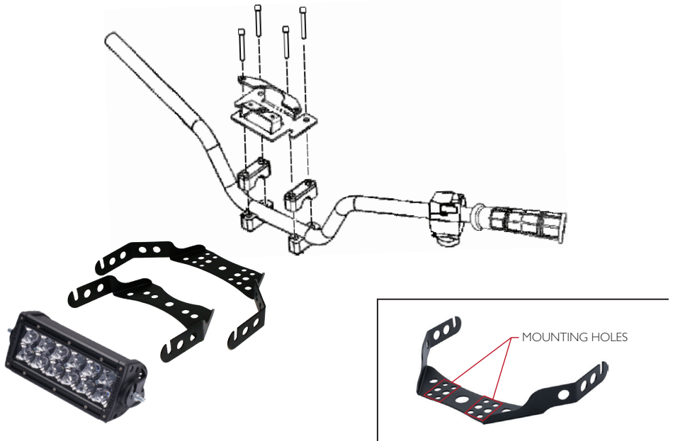
Figure 1. Mounting Bracket
